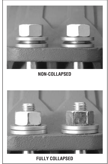
Figure B — COLLAPSIBLE WASHERS
