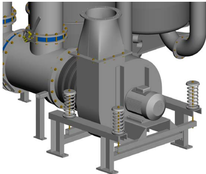
A blower unit mounted on VTV2G/35-1500A Ground Shock Isolators
