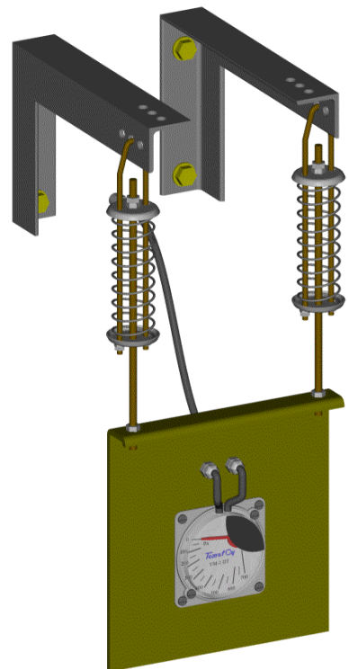
Example of shock isolation of light weight equipment using VTV2G/35-50B Ground Shock Isolators
