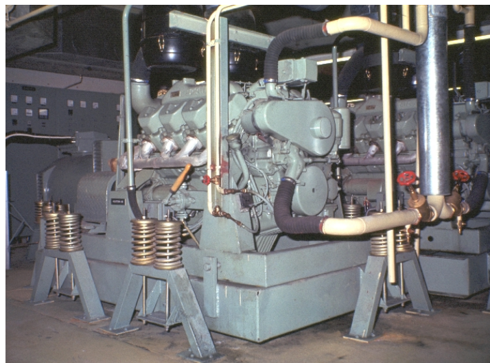
A diesel generator mounted on VTV2G/35- 6000 A Ground Shock Isolators.
