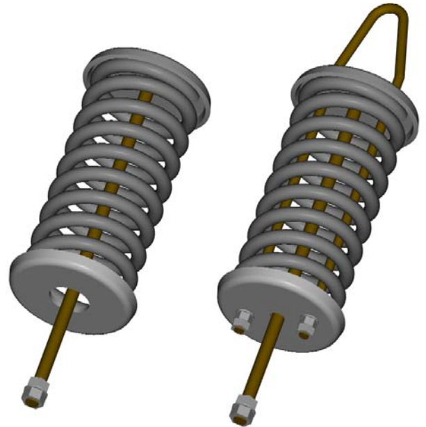
VTV2G/35-6000A and -6000B Ground Shock Isolators
