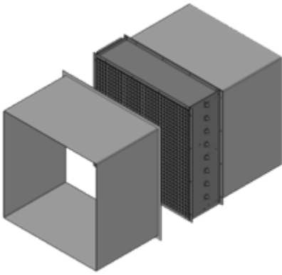
HV-Series damper installed in duct
