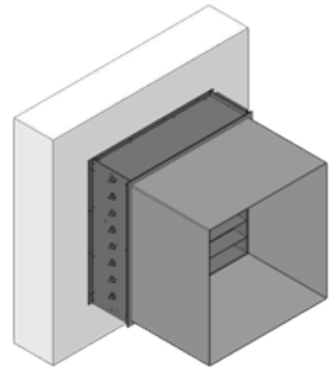
HV-Series damper installed inside of blast resistant wall and connected to duct
